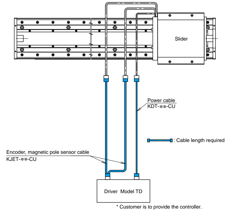
Specifications with the magnetic pole sensor
