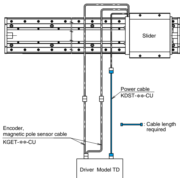
Specifications with the magnetic pole sensor
