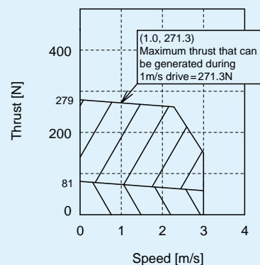
Fig.2 Thrust-speed characteristics chart (Motor attraction force is included)
