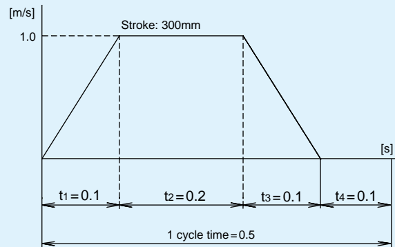
Fig.1 Motion profile
