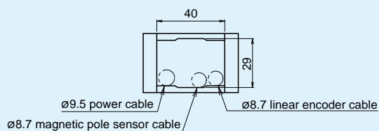
Cross section of the cable carrier
