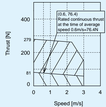
Fig.4 Thrust-speed characteristics chart (Motor attraction force is included)
